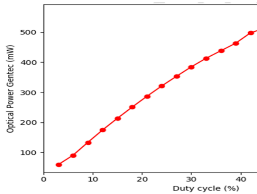
Typical average optical power of the laser as a function of the laser duty cycle with a pulsewidth of 900ns and a base plate temperature of +20°C
