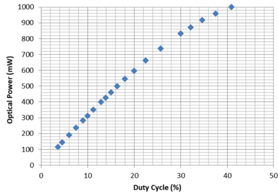
Typical average optical power of the laser as a function of the laser duty cycle with a pulsewidth of 900ns and a base plate temperature of +20°C
