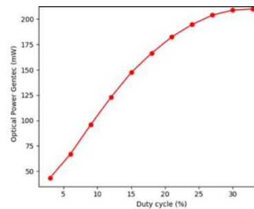
Average optical power of the laser as a function of the laser duty cycle with a pulsewidth of 900ns and a laser temperature of +20°C
